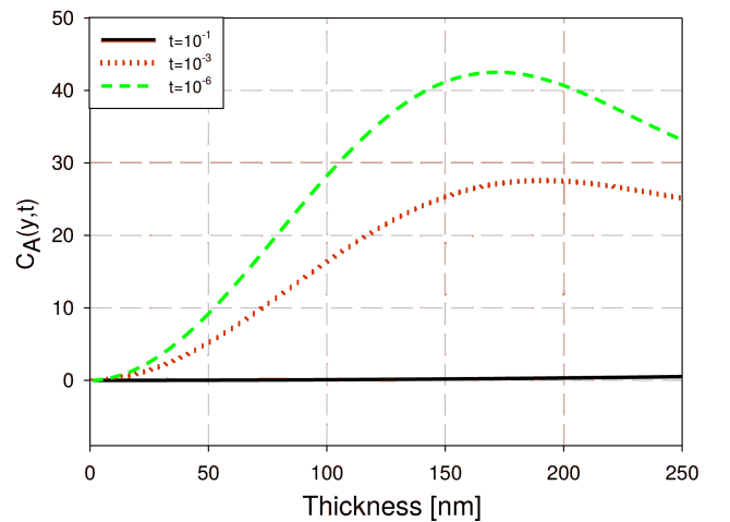
Fig. 4. Profiles of the concentration of gaseous molecules depending on the thickness of the layer in time t = 10^{-6}, 10^{-3}, 10^{-1} s, at C_S = 10000 ppm, n = 6 , k_D = 10^6 s ^{-1} , D_K = 10^6 nm ^2 s ^{-1} .
