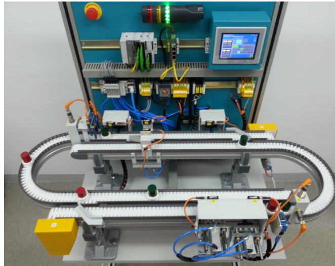
Fig. 3. The physical model of mobile teaching stand for e-learning of PLC programming for conveyor engineering
