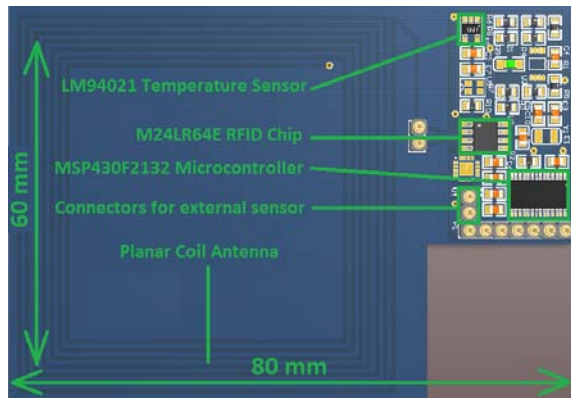
Fig. 1. Prototype board of the platform with main elements and external dimensions marked
