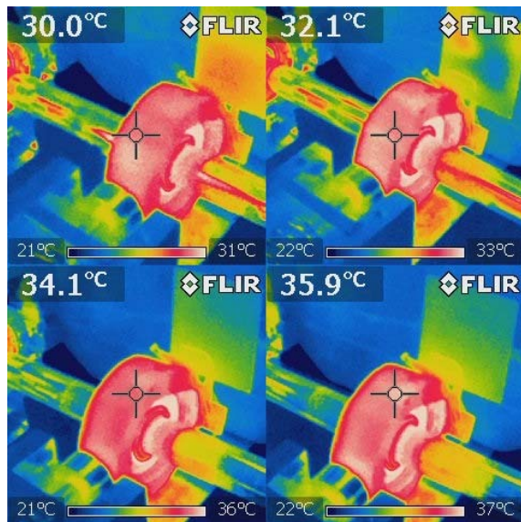
Fig. 4. Temperature data collected by the using of FLIR i7 infrared camera
