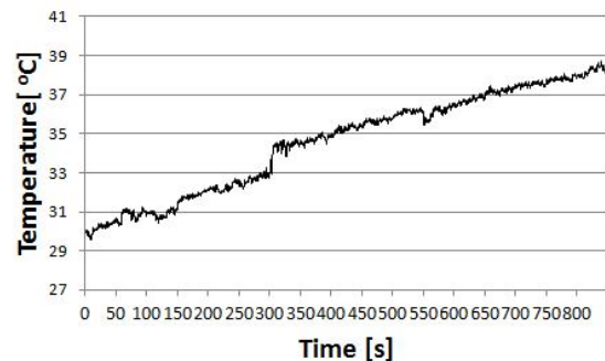
Fig. 3. Temperature data collected by the using of wireless sensing platform
