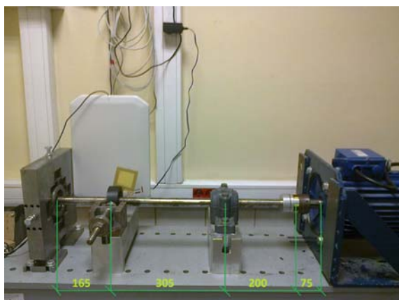
Fig. 2. Laboratory test-stand with the sensing system installed
