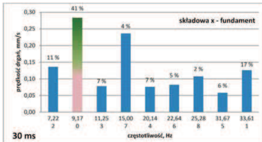
Rys. 21. Histogram atomów Gabora – analiza MP drgań fundamentu – opóźnienia 30 ms Fig. 21. Histogram of Gabor molecules – the MP analysis for the vibrations recorded on the structure foundation – time delays 30 ms
