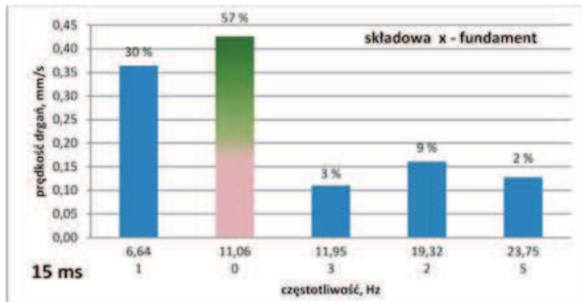
Rys. 20. Histogram atomów Gabora – analiza MP drgań fundamentu – opóźnienia 15 ms Fig. 20. Histogram of Gabor molecules – the MP analysis for the vibrations recorded on the structure foundation – time delays 15 ms
