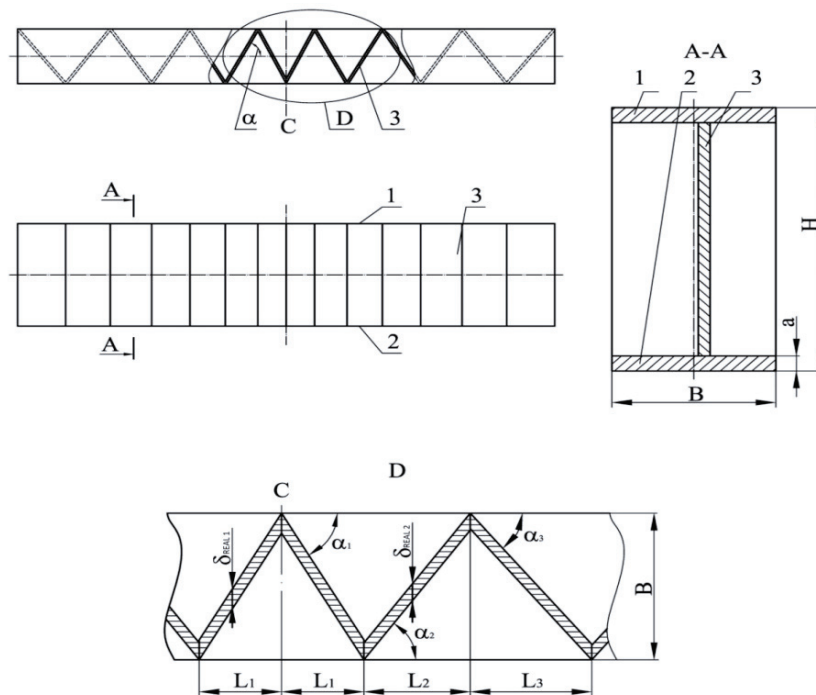
Fig. 4. Span beam [7, 8]
