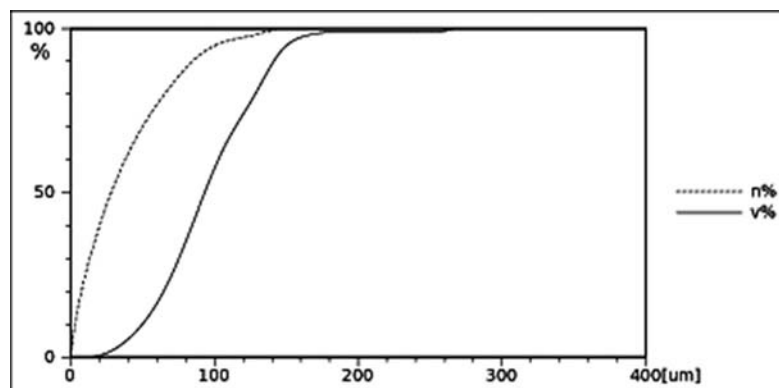
Fig. 6. Cumulative distribution of droplet spectra for the urea solution with the addition of nigrosine with setting d_1 (v% – mass, n% – number of droplets)
