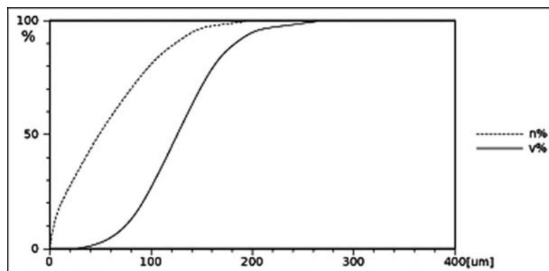
Fig. 5. Cumulative distribution of droplet spectra for the nigrosine solution with setting d_5 (v% – mass, n% – number of droplets)
