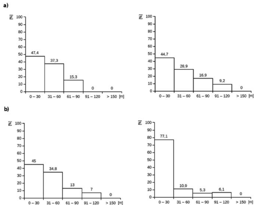
Fig. 3. Percentage distribution of the field dose in the 30 meter strip: a) setting d_1 , left – liquid N, right – liquid M, b) setting d_5 , left – liquid N, right – liquid M
