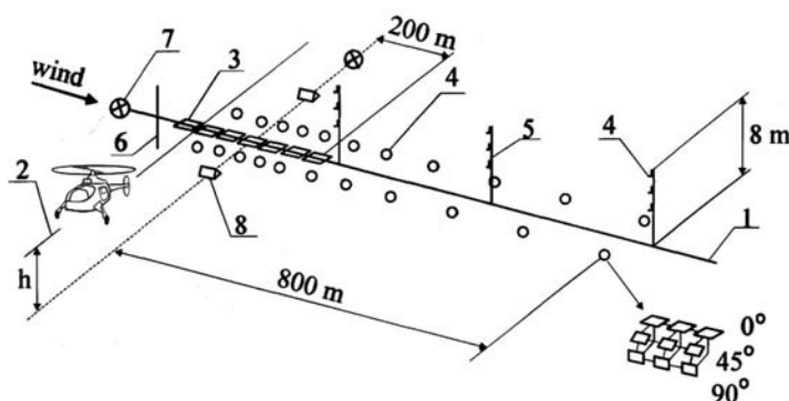
Fig. 1. The schematic drawing of the research experiment site and the measurement line: 1 – measure line, 2 – flight path, 3 – mass samplers, 4 – droplet samplers, 5 – masts, 6 – measurements of meteorological parameters, 7 – cameras, 8 – markers
