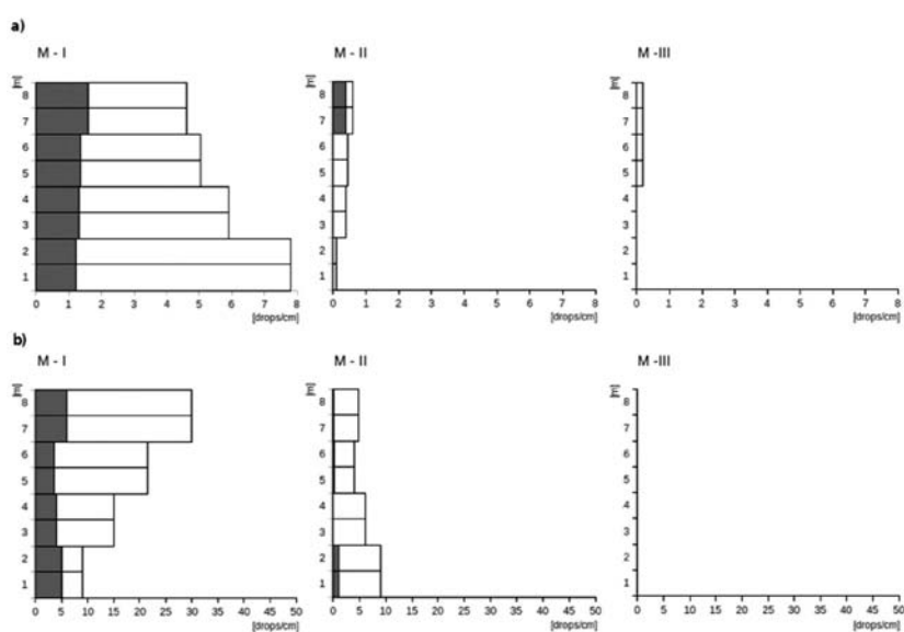
Fig. 8. Density distribution of the spray on masts for the nigrosine solution (gray color – horizontal samplers, white color – vertical samplers): a) setting d_1 , b) setting d_5
