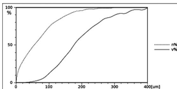
Fig. 7. Cumulative distribution of droplet spectra for the urea solution with the addition of nigrosine with setting d_5 (v% – mass, n% – number of droplets)
