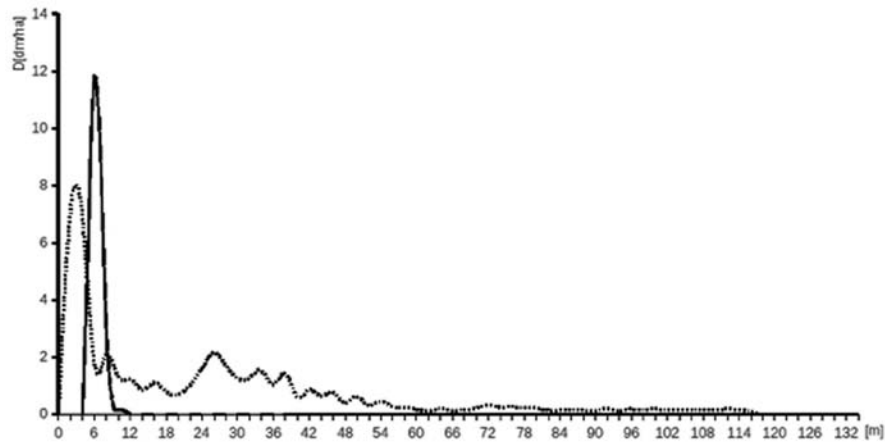
Fig. 2. Averaged distribution of the sprayed mass of liquid M: solid line – theoretical distribution [13], dotted line – setting d_5
