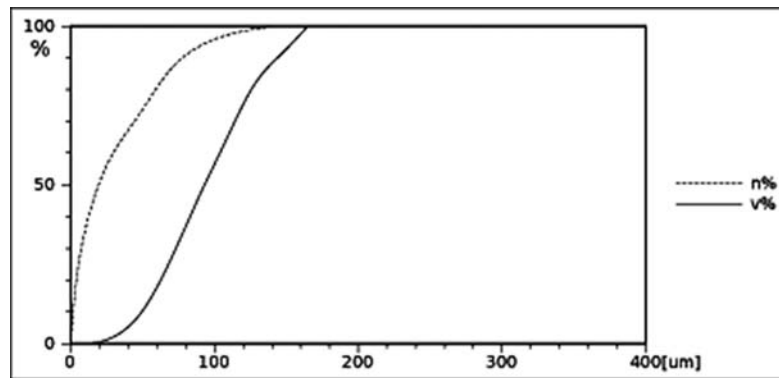
Fig. 4. Cumulative distribution of droplet spectra for the nigrosine solution with setting d_1 (v% – mass, n% – number of droplets)
