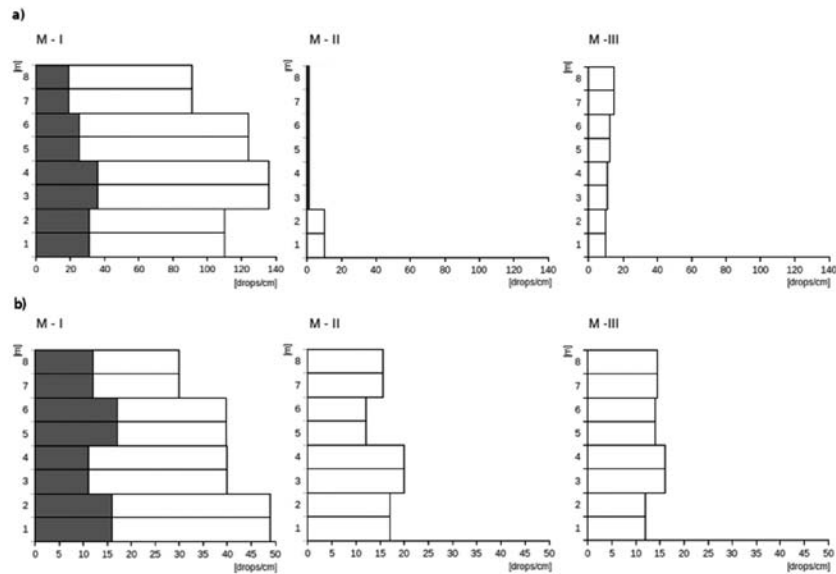
Fig. 9. Density distribution of the spray on masts for the urea solution with the addition of nigrosine (gray color – horizontal samplers, white color – vertical samplers): a) setting d_1 , b) setting d_5
