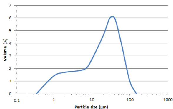
Fig. 1. Volumetric particle size distribution of feed sample
