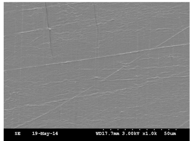
Fig. 3. a) The SEM's image of the first cracks around "inclusions" in the polyurethane in the micro-shear test for the sample nr 1 from Table 1 (force 6 N). b) The SEM's image of the first cracks in the micro-shear test for the sample nr 1 from Table 1 (force 7 N)
