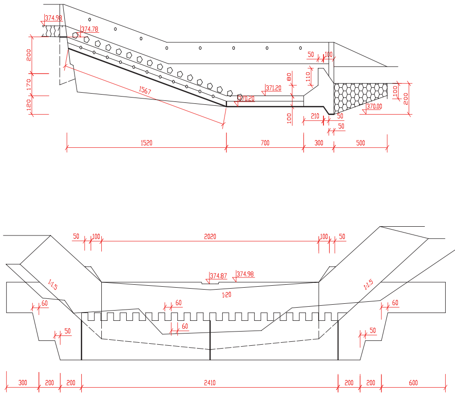
Figure 4. The block ramps structure designing plots
