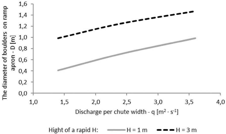
Figure 1. A diagram for choosing the dimension of boulder to install it on block ramp
