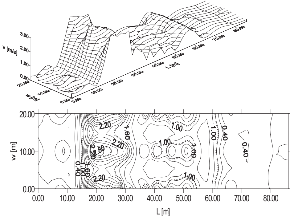
Figure 3. Water velocity values for a sloping block ramp apron and for the upstream curtain wall part of the river channel upstream of the block ramp hydraulic structure
