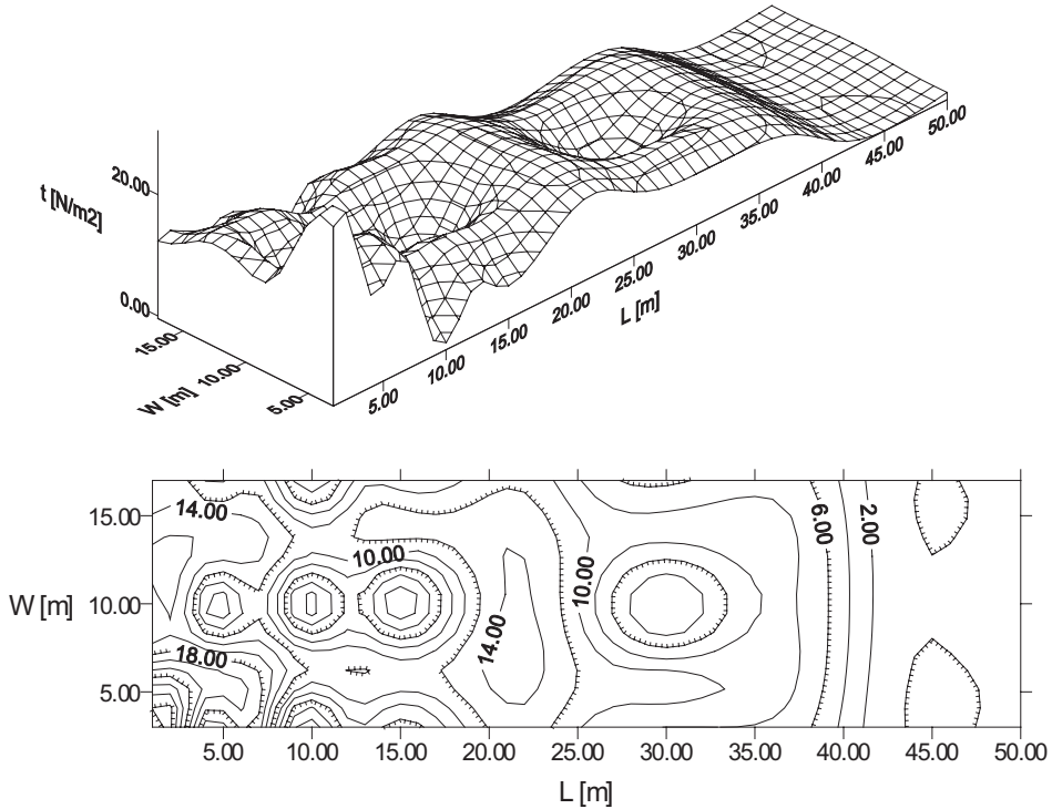
Figure 2. Shear stress values for the river bed upstream of the upstream curtain wall of the block ramp hydraulic structure
