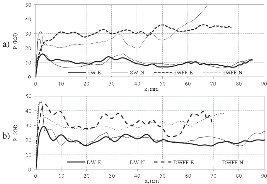
Fig. 8. Instantaneous crushing force from finite element analysis (N) and from the experiments (E) of (a) SW and SWFF column, and (b) DW DWFF column
