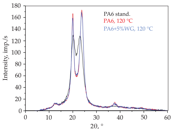
Fig. 4. Comparison of WAXS patterns of: standard PA6 fibers (black curve), PA6 fibers treated at 120 °C (red curve) and modified in the bath (WG 5 wt %) at 120 °C (blue curve), respectively
