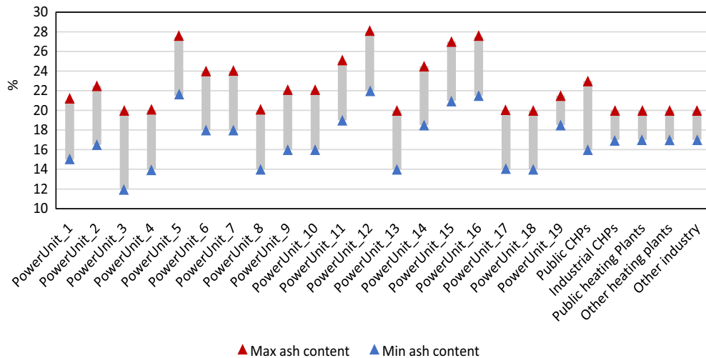
Fig. 6. Minimal and maximal ash content in fine coal required by demand units (%)
