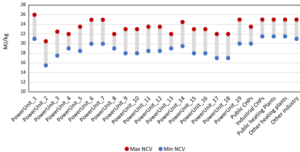
Fig. 5. Minimal and maximal NCV of fine coal required by demand units (MJ/kg)
