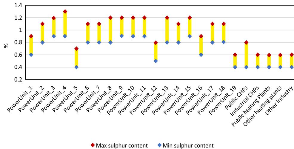
Fig. 7. Minimal and maximal sulphur content in fine coal required by demand units (%)
