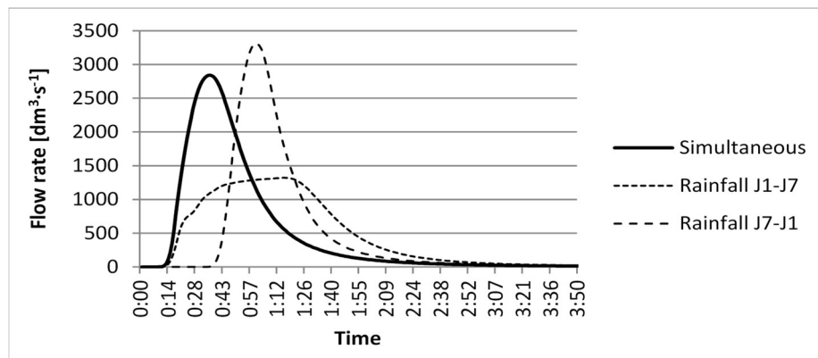
Fig. 6. Outflow from the catchment - rain wave speed 50 \text{ m} \cdot \text{min}^{-1} - rainfall frequency F = 2 years
