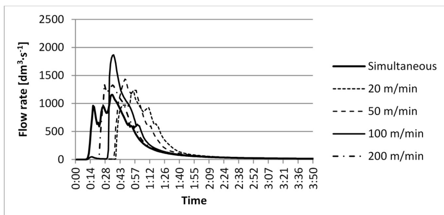
Fig. 10. Outflow from real catchment - rainfall frequency F = 2 years
