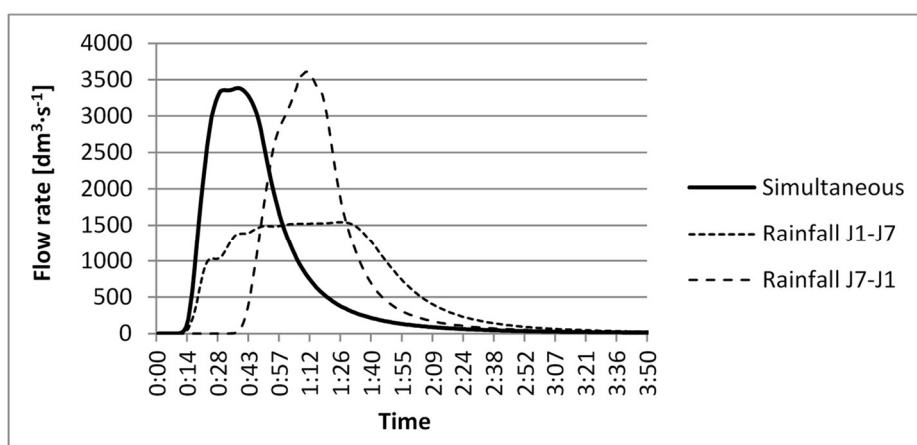
Fig. 5. Outflow from the catchment - rain wave speed 20 \text{ m} \cdot \text{min}^{-1} - rainfall frequency F = 3 years
