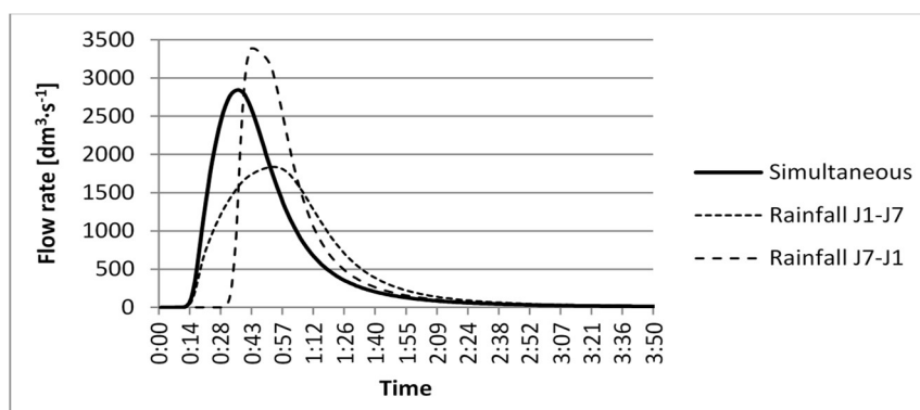
Fig. 8. Outflow from the catchment - rain wave speed 100 \text{ m} \cdot \text{min}^{-1} - rainfall frequency F = 2 years
