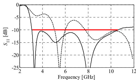
Fig. 2. The reflection response of the proposed UWB slot antenna at the initial (---) and the optimized (—) design.
