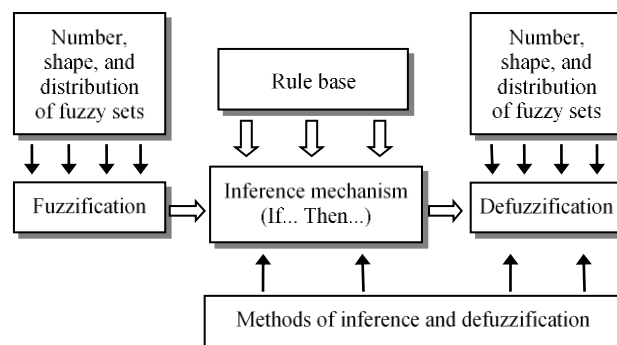
Fig. 4 Structure of fuzzy system
