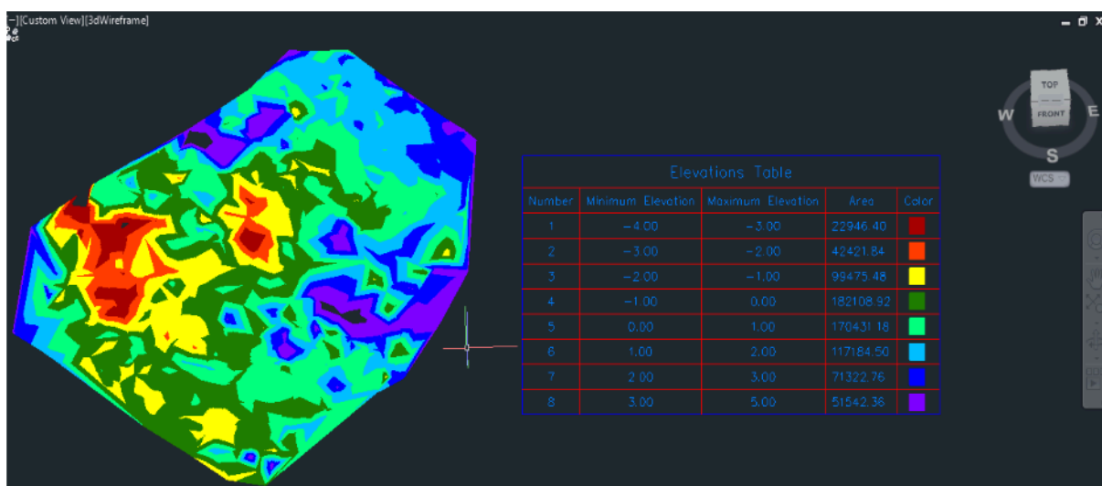
Fig. 9. Compared Z displacement between the data before the land sliding happened on 2007 (using Plaxis 3D analyses) and the data after the land sliding happened on 2022 (using the drone data analyses)
