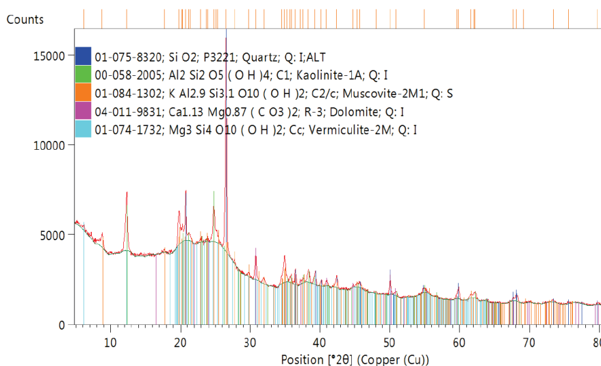
Fig. 3. X-ray diffraction pattern of coal sample with the identification of crystalline phases
