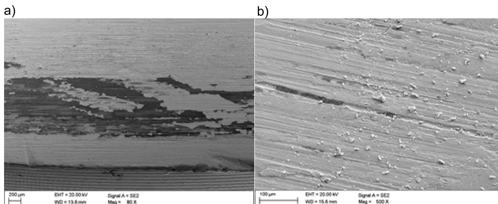
Fig. 6a, b. SEM micrographs of the surface of the steel sample after wear tests using hard coal
