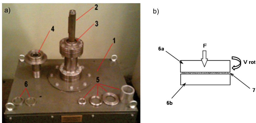
Fig. 4. Test stand: a – site view, b – carbon abrasive load model
