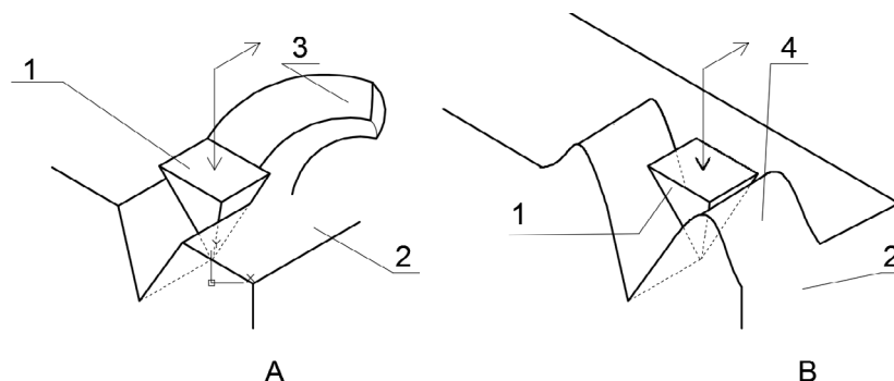
Fig. 2. Schematic representation of elementary mechanisms of abrasive wear A – micro-cutting, B – micro-ploughing; 1 – abrasive particle, 2 – surface being worn, 3 – separated cut, 4 – ridge (Zum Gahr 1987)
