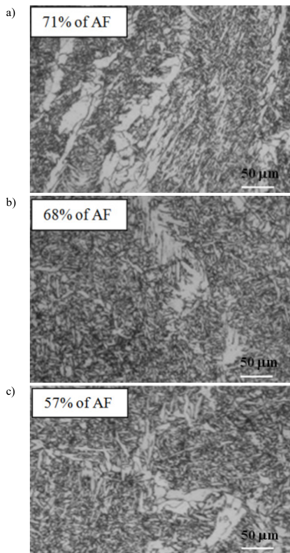
Fig. 3. Microstructure of WMD after MAG welding with micro-jet cooling gas: a) Ar-steam diameter 50 \mu\text{m} , b) Ar-steam diameter 40, c) 50% Ar/50 % Air-steam diameter 40 \mu\text{m} \mu\text{m} 200x
