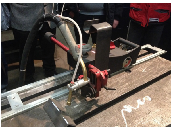
Fig. 1. MIG welding head with micro-jet injector
