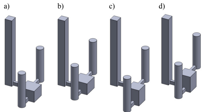
Fig. 2. Schema of the gating system configuration low reaction chamber N, fed into the top (a) fed into the bottom (b) and high reaction chamber W fed into the top (c) fed into the bottom (d)
