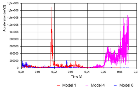
Fig. 13. Time processes of acceleration in models 1, 4 and 6
