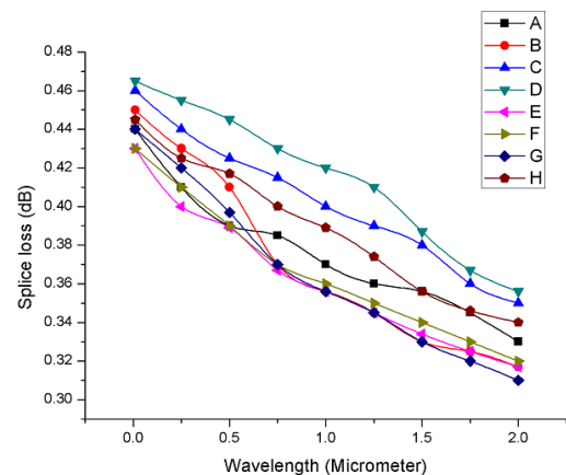
Fig. 5. Splice loss
