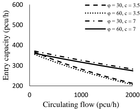
(a) Inscribed circle diameter = 20m, Approach width = 3.5m
