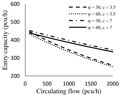
(c) Inscribed circle diameter = 50m, Approach width = 3.5m
