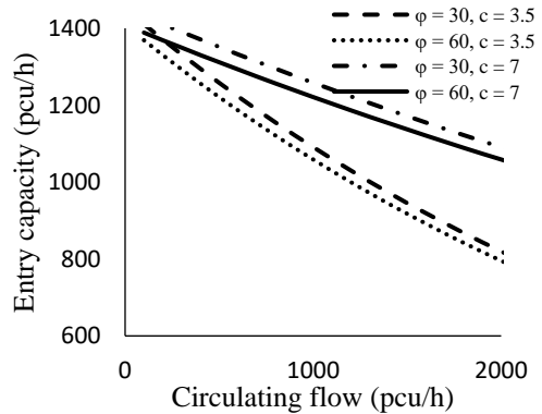
(d) Inscribed circle diameter = 50m, Approach width = 7m
