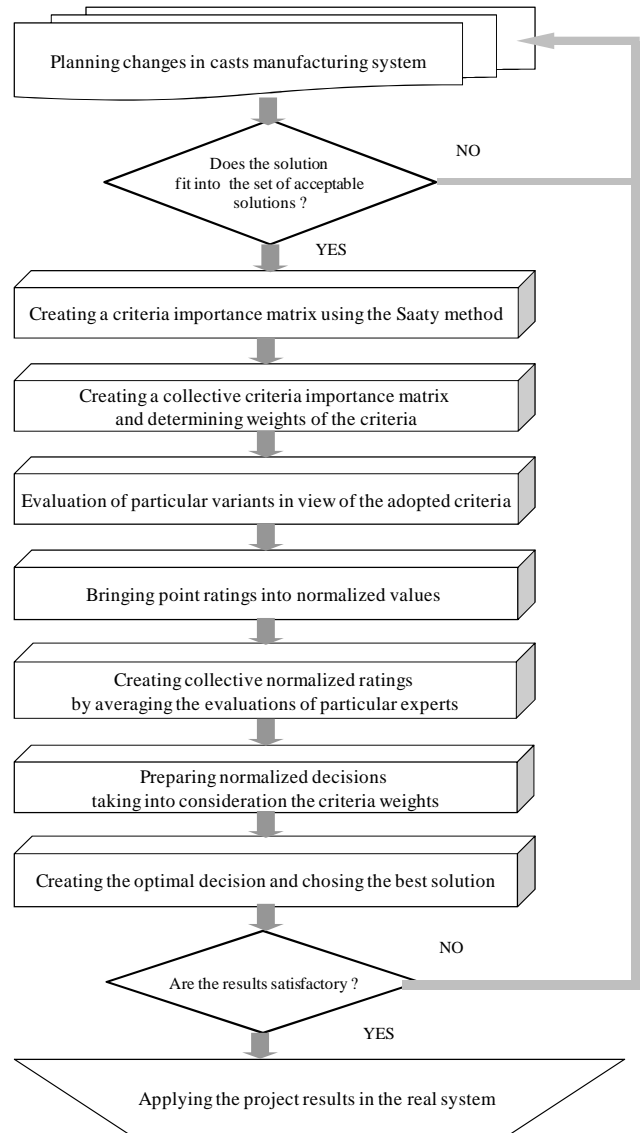
Fig. 2. Multi-criterion valuation of variants according to Yager's method
