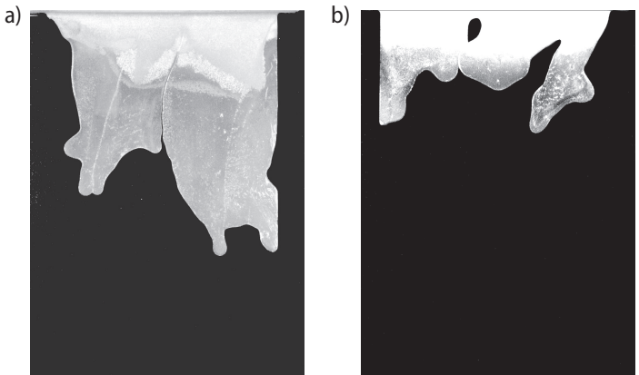
Fig. 3. Effect of casting temperature on fluidity: a) setup 5–1.5 mm, top gated, T_{POUR} 1700°C, T_{mold} 900°C; b) setup 1–1.5 mm, top gated, T_{POUR} 1550°C, T_{mold} 900°C
