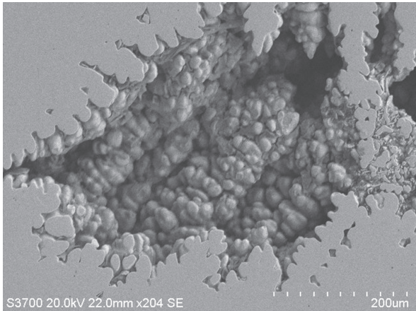
Fig. 12. SEM images showing large shrinkage pores in top-gated sample from Set-up 7
