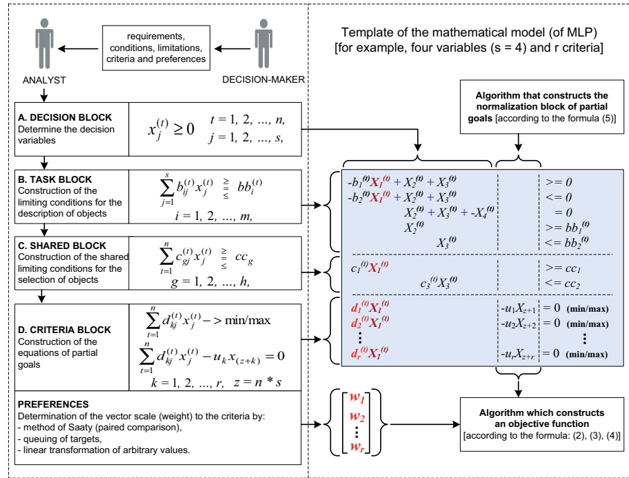
Fig. 3. The idea of constructing a pattern (template) of the mathematical model (source: [2])
