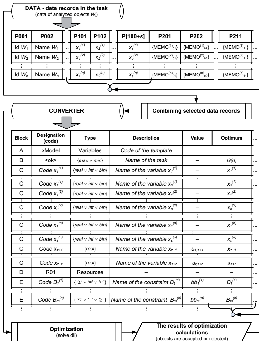
Fig. 5. The procedure of transformation of data records to the matrices of a multi-model (so-called converter) in the system supporting decision-making (source: [2])
