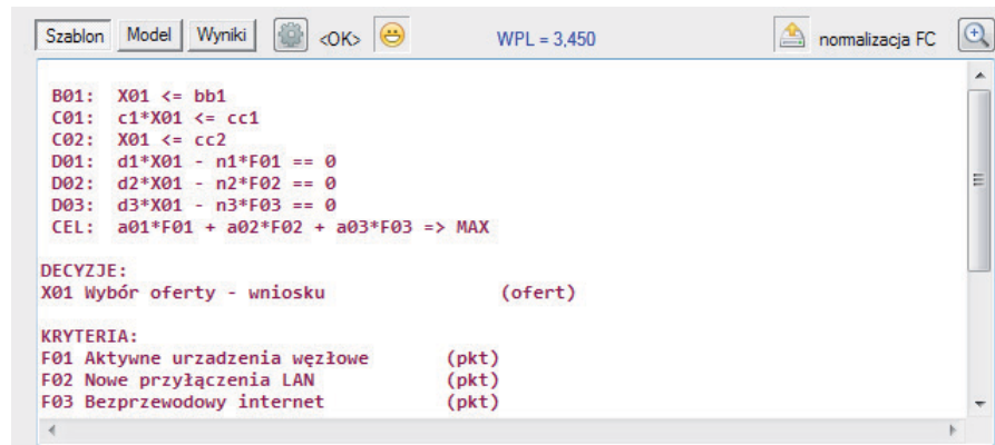
Screen 1. Decision problem described in the algebraic form – form M1 (source: system DSS 2.0)
