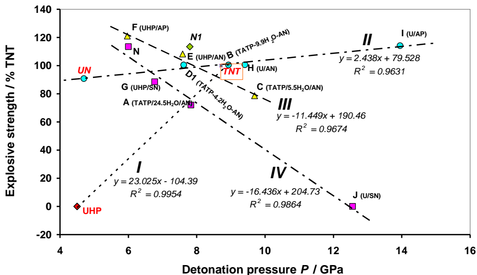
Fig. 1. Mutual relationship between experimental relative explosive strength and calculated detonation pressure of the studied mixtures
