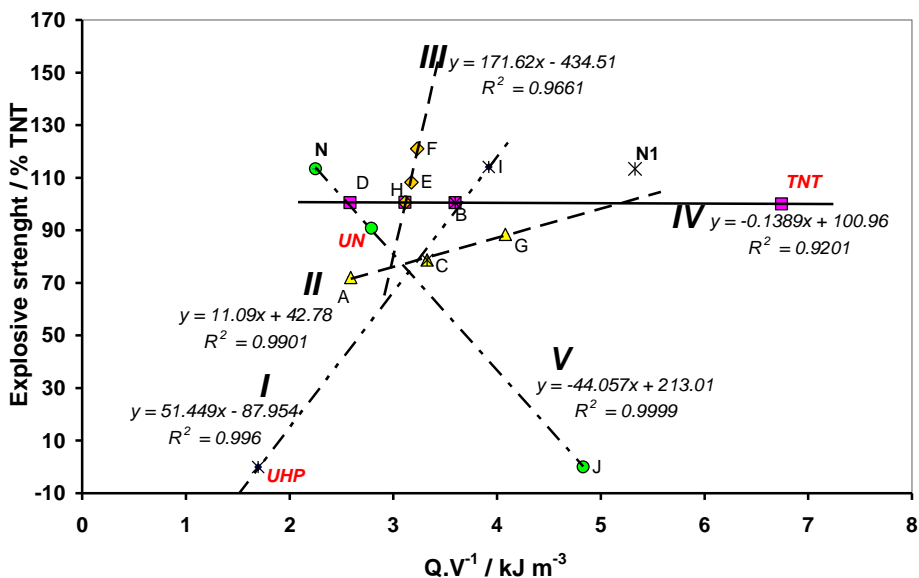
Fig. 2. Mutual relationship between experimental relative explosive strength and heat content of the gaseous products ( Q.V^{-1} ) of the studied mixtures detonation.
