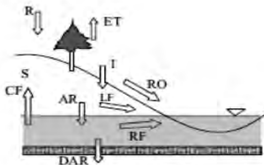
Fig. 1. Schematic illustration of the conceptual water balance model in SWAT; R = rainfall, ET = evapotranspiration, I = infiltration, RO = runoff, RF = return flow, LF = lateral flow, CF = capillary flow, AR = aquifer recharge, DAR = deep aquifer recharge, S = soil moisture; source: own elaboration
