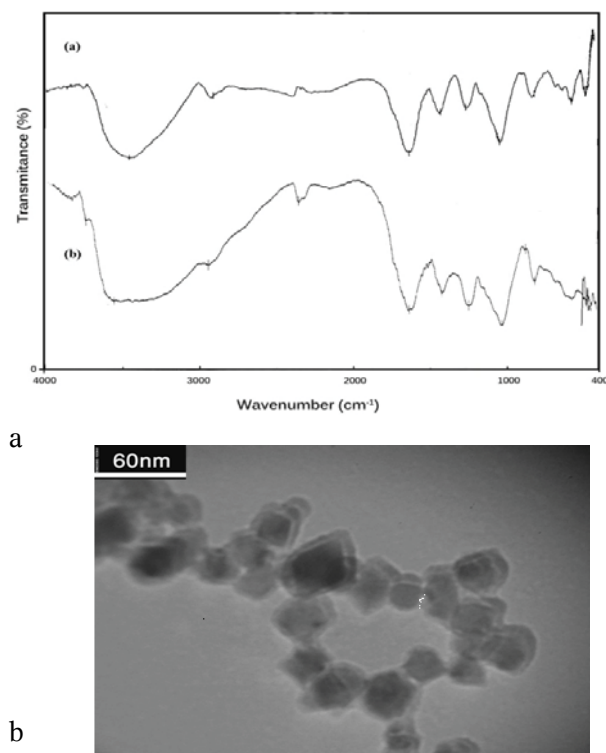
Fig. 1. (a) FTIR spectra of irradiated Ergosan extract (alginate) (a) and crude Ergosan extract (alginate) (b); (b) TEM image of Ergosan extract (alginate) after irradiation.
