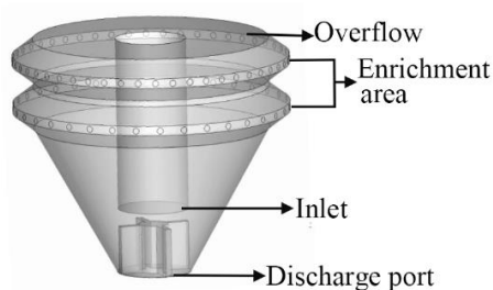
Fig. 3. Structure of the Falcon concentrator
