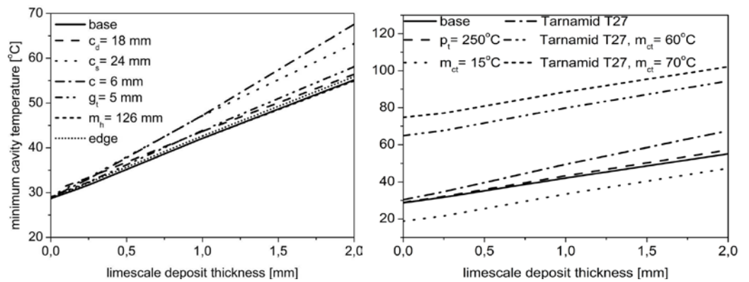
Fig. 3. Graph of the minimum temperature on the molding cavity surface
