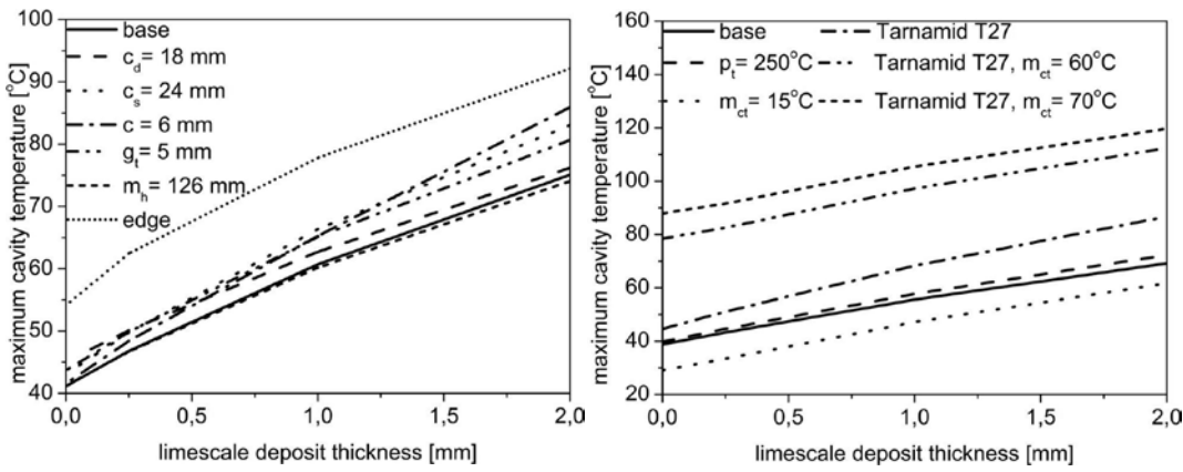
Fig. 4. Graph of the maximum temperature on the molding cavity surface
