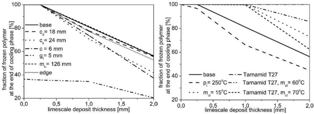
Fig. 7. Graph of the frozen plastic fraction at the end of the cooling phase
