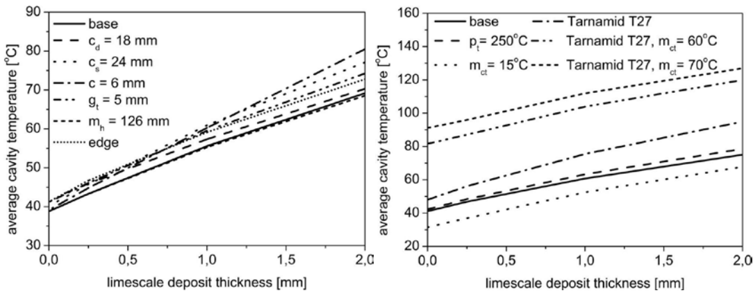
Fig. 2. Graph of the average temperature on the molding cavity surface
