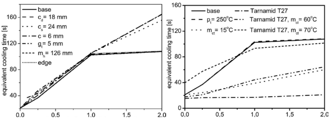
Fig. 8. Graph of the equivalent cooling time, in which the entire plastic material becomes solidified and the mold achieves the assumed cavity temperature.
