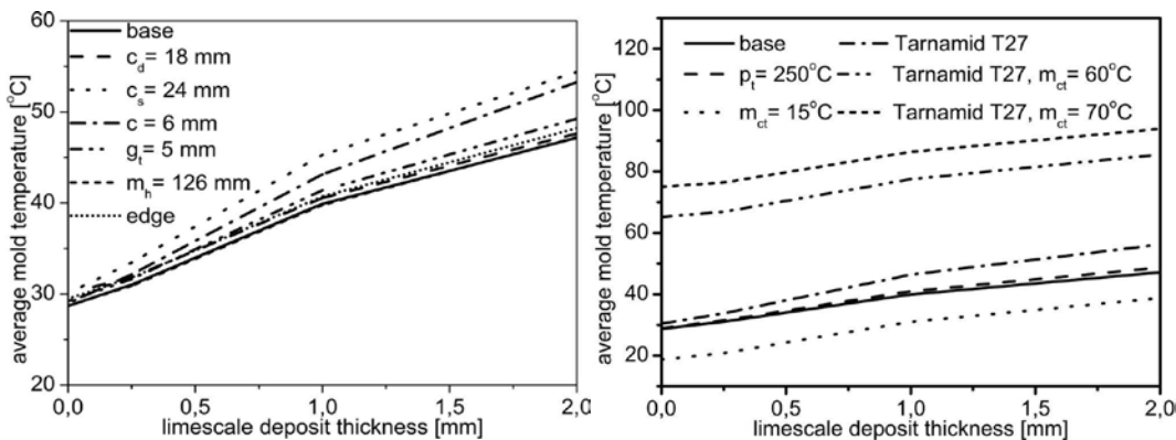
Fig. 6. Graph of the average injection mold temperature
