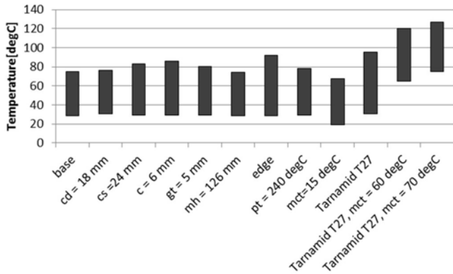
Fig. 5. Graph of the minimum and maximum temperature on the molding cavity surface for a scale deposit layer of 2 mm
