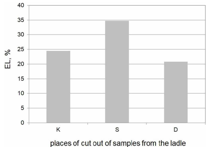
Fig. 11. Results of elongation (EL) depending on places where samples were cut from slag ladle: K – flange; S – half-height of ladle; D – bottom of ladle
