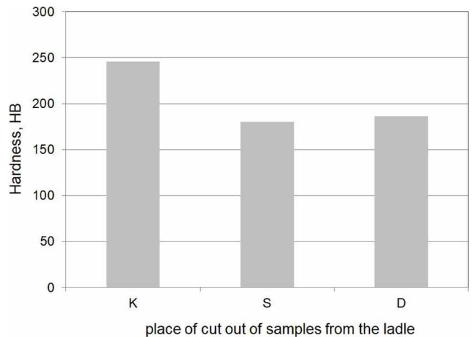
Fig. 9. Change in hardness depending on places where sample was cut from slag ladle: K – flange; S – half-height of ladle; D – bottom of ladle; (average of four measurements)
