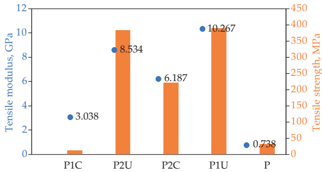
Fig. 4. Tensile properties of the samples
