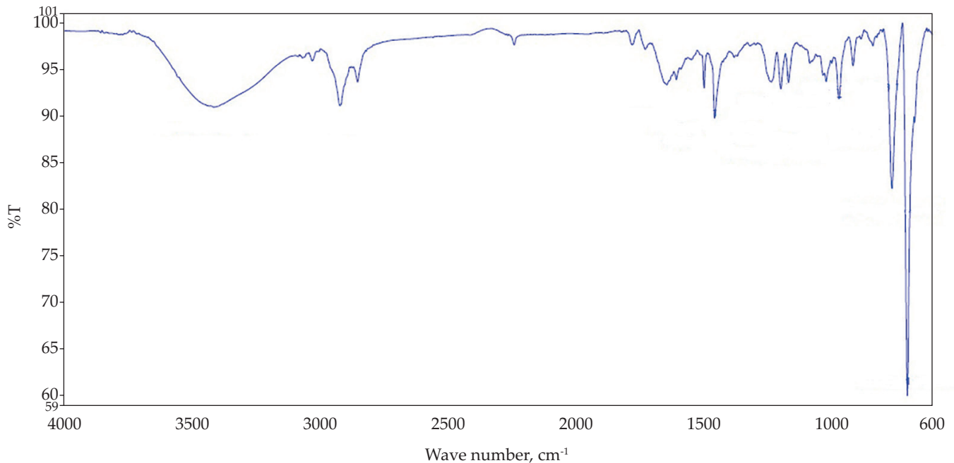
Fig. 3. FTIR spectra of car side mirror cover
