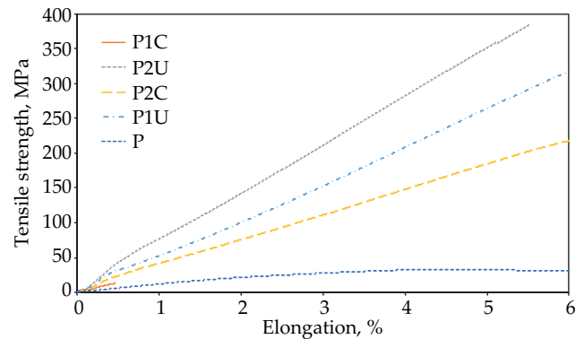
Fig. 5. Stress-strain curves of the samples
