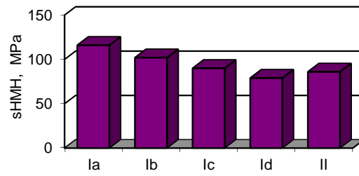
Fig. 7. The maximum values \sigma_{\text{HMH}} of the stress in the plate
