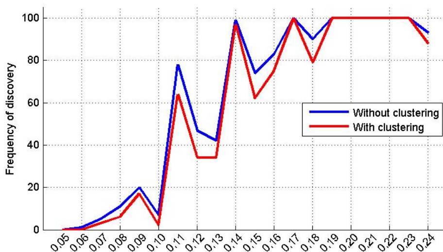
Fig. 1: Frequency of detection of causal SNPs with clustering (mBIC2 with p_C ) and without clustering (mBIC2 with p ), where I_S = 2000 .
