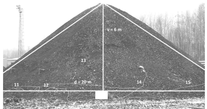
Fig. 1 Experimental heap No. V at TUM Sokolov stack – injected measuring probes
