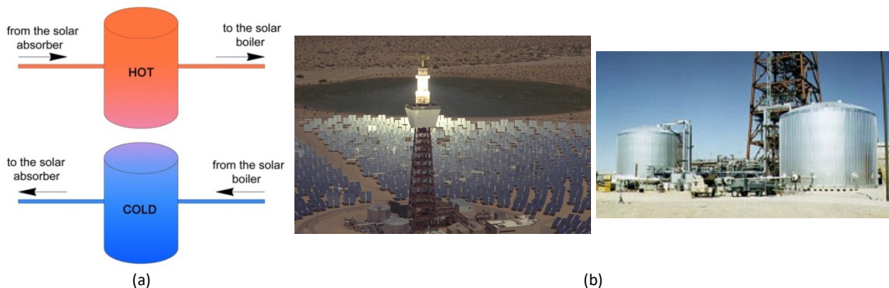
Fig. 5. Illustration of the direct concept applied for HT heat storage with molten salt in CSTP plant: (a) Two-tank direct heat storage concept; (b) The two-tank direct molten-salt TES system at the Solar Two CSTP plant.
