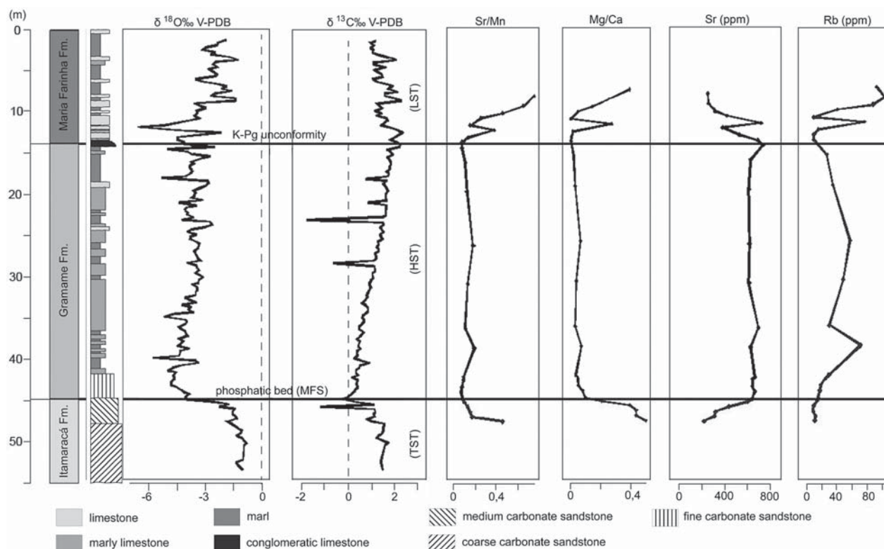
Fig. 7. Trends in oxygen and carbon isotopes, and Mn/Sr, Mg/Ca, Sr and Rb values in the Poty Quarry.
