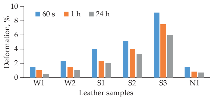
Fig. 1. Deformation of samples in the parallel direction for 100 h irradiation cycle
