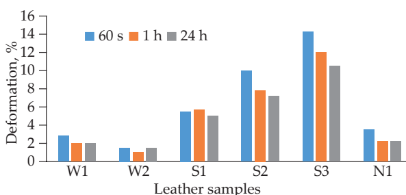
Fig. 5. Deformation of samples in the perpendicular direction for 150 h irradiation cycle
