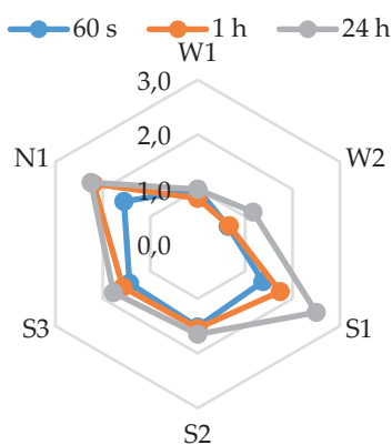
Fig. 3. Anisotropy phenomenon as a dependence of time after the force removal for 100 h irradiation cycle
