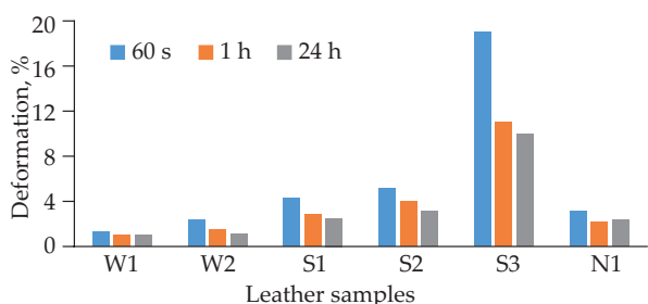
Fig. 4. Deformation of samples in the parallel direction for 150 h irradiation cycle
