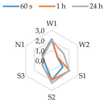
Fig. 6. Anisotropy phenomenon as a dependence of time after the force removal for 150 h irradiation cycle
