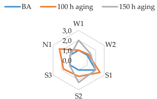
Fig. 7. Anisotropy coefficient before (BA) and after aging during 100 and 150 hours
