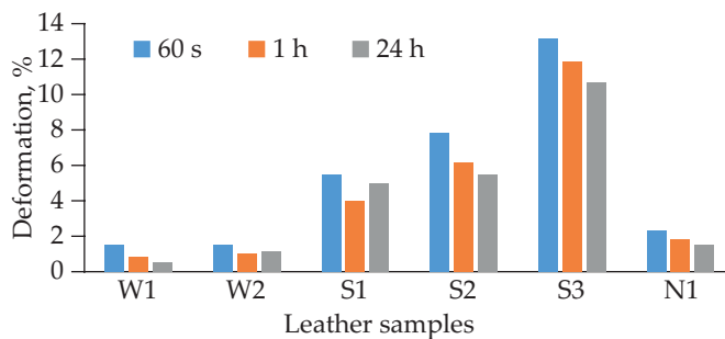
Fig. 2. Deformation of samples in the perpendicular direction for 100 h irradiation cycle
