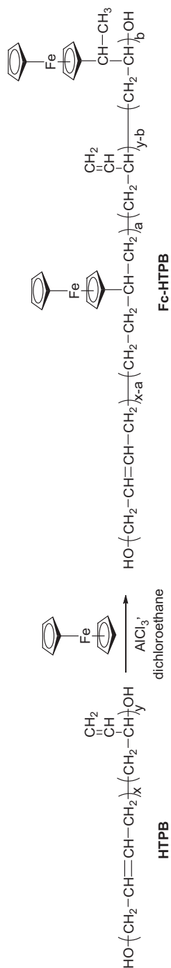
Scheme 11. Introduction of ferrocene groups onto HTPB via Friedel-Crafts reaction
