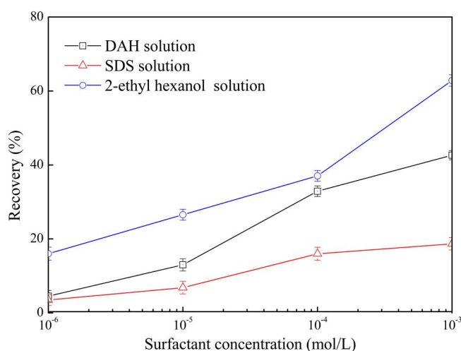
Fig. 6. Recovery of low-rank coal samples as a function of 2-ethyl hexanol, DAH and SDS concentrations
