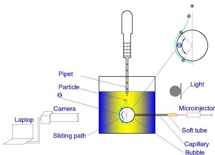
Fig. 3. A schematic of sliding interaction between a particle and a bubble in flotation
