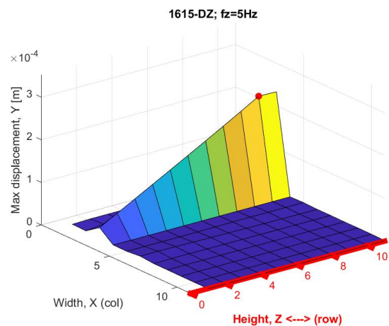
Fig. 15. Amplitudes of vibration displacements in the Z direction, excitation force in the Z direction
