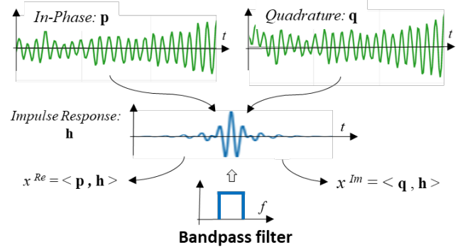
Fig. 5. The proposed range-filtering scheme employing dot products between In-Phase and Quadrature components of radar-produced data (represented by vectors \mathbf{p} and \mathbf{q} ) and filter impulse response ( \mathbf{h} )
