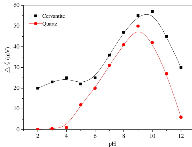
Fig. 7. Effect of pH on zeta potential difference of minerals before and after treatment with sodium oleate
