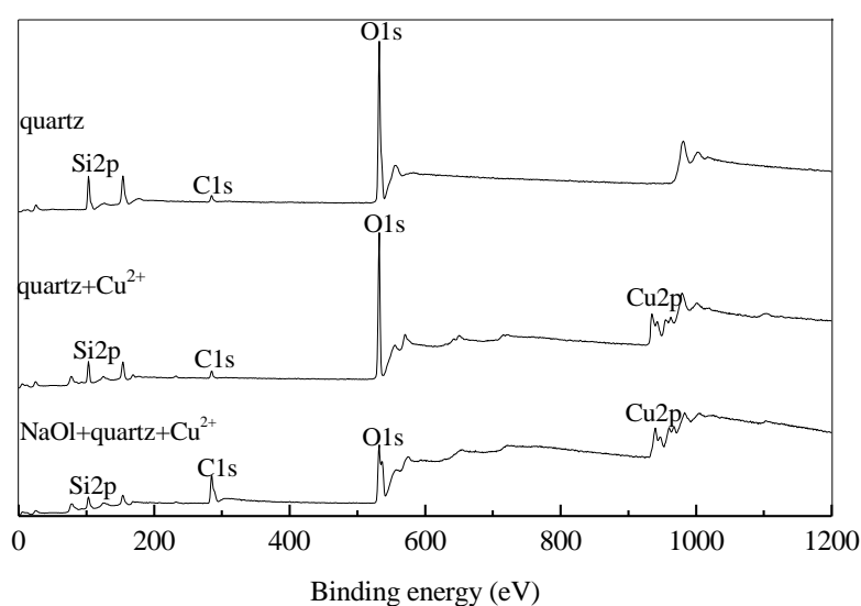
Fig. 12. XPS spectrogram of quartz before and after treatment with copper ions and sodium oleate at pH 6.0
