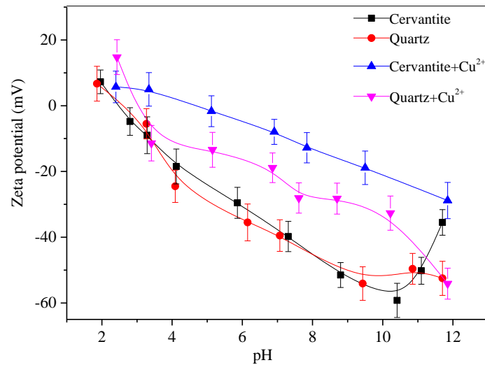
Fig. 5. Effect of pH on zeta potential of minerals before and after treatment with \text{Cu}^{2+} ( \text{Cu}^{2+} 5 \times 10^{-4} \text{ M} )
