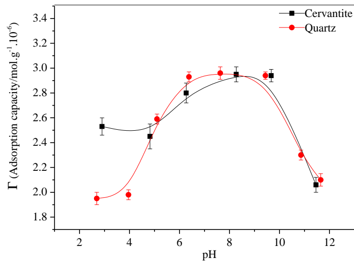
Fig. 9. Effect of pH on the adsorption capacity of sodium oleate on minerals in the presence of Cu 2+
