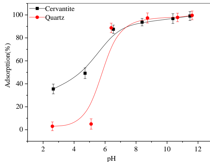
Fig. 4. Effect of pH on the adsorption of \text{Cu}^{2+} on mineral surfaces
