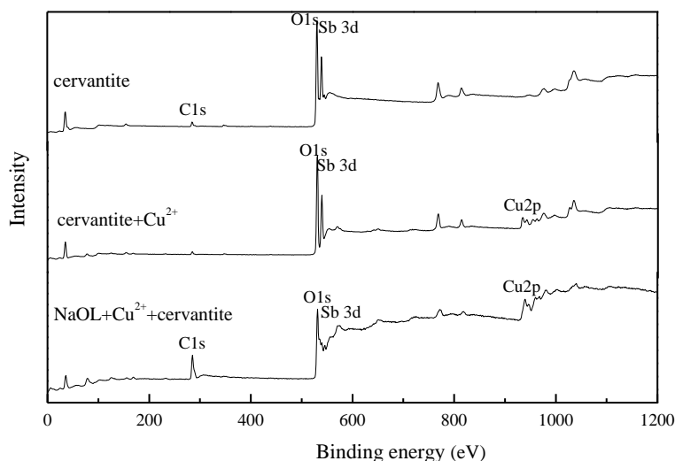
Fig. 11. XPS spectrograms of cervantite before and after treatment with copper ions and sodium oleate at pH 6.0
