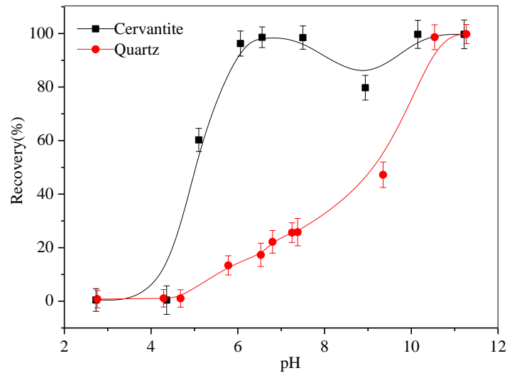
Fig. 3. Effect of pH on mineral recovery using sodium oleate as a collector and \text{Cu}^{2+} as an activator (sodium oleate 1.5 \times 10^{-4} M; \text{Cu}^{2+} 5 \times 10^{-4} M)
