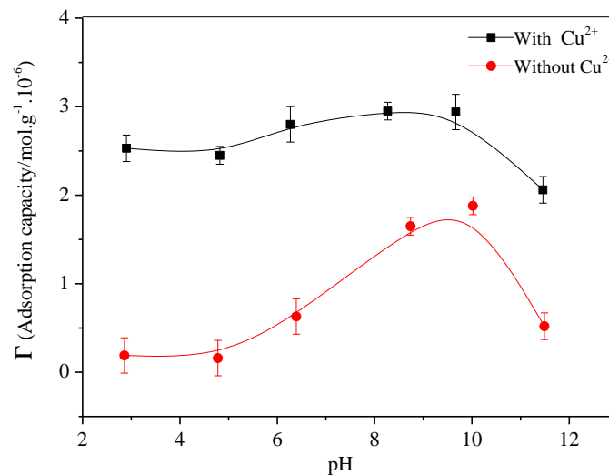
Fig. 8 Relationship between pH and adsorption capacity of sodium oleate on cervantite, with or without \text{Cu}^{2+}
