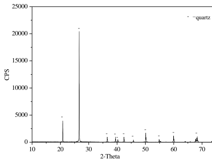
Fig. 2. XRD diffraction pattern of quartz
