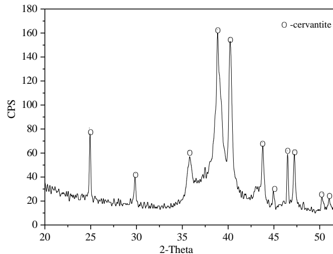
Fig. 1. XRD diffraction pattern of cervantite
