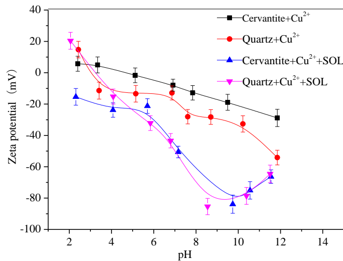
Fig. 6. Effect of pH on zeta potential of minerals before and after treatment with sodium oleate ( \text{Cu}^{2+} 5 \times 10^{-4} \text{ M} , sodium oleate 1.5 \times 10^{-4} \text{ M} )
