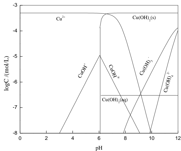
Fig. 10. The logC-pH diagram for hydrolysis species of Cu ions
