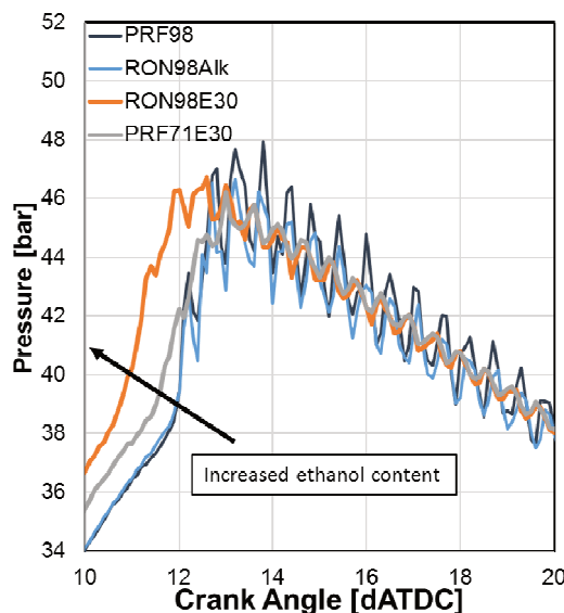
Fig. 10. Closer examination of the cylinder pressure behavior just after the knock-point
