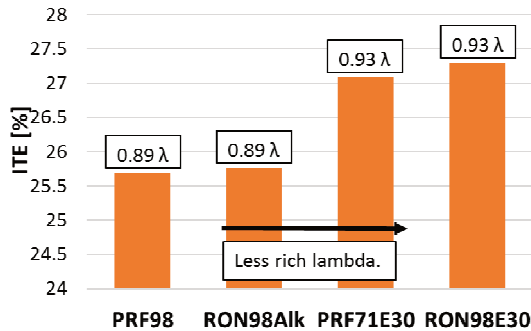
Fig. 5. Indicated thermal efficiency of each fuel at RON test conditions
