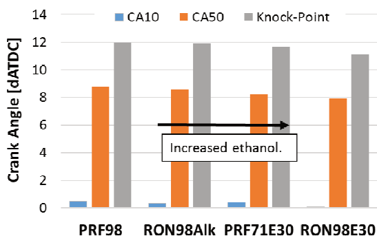
Fig. 9. Crankshaft angle position at 10% mass fraction burned (CA10), 50% (CA50), and the knock-point for all fuels at RON rating conditions
