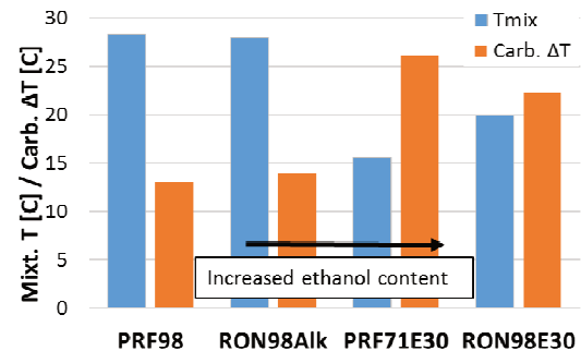
Fig. 3. Mixture temperature after the carburetor and corresponding temperature drop across the carburetor
