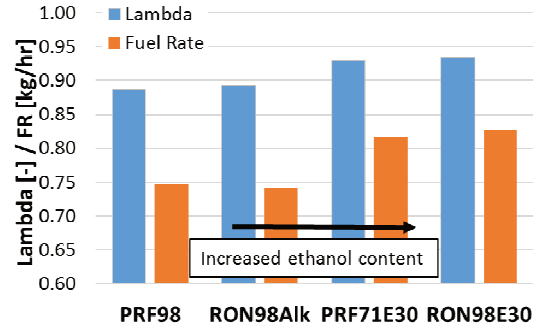
Fig. 2. Lambda and fuel rate (FR) at RON rating conditions for each fuel
