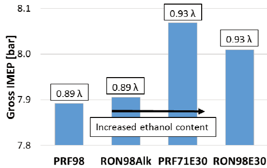
Fig. 4. Effect of fuel properties on engine load during RON testing
