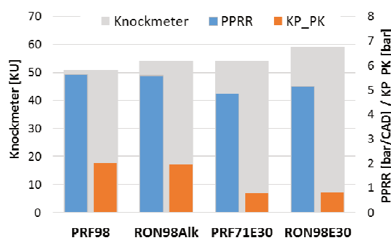
Fig. 11. Comparison of ASTM knockmeter measurement, peak pressure rise rate (PPRR), and knocking pressure peak (KP_PK)
