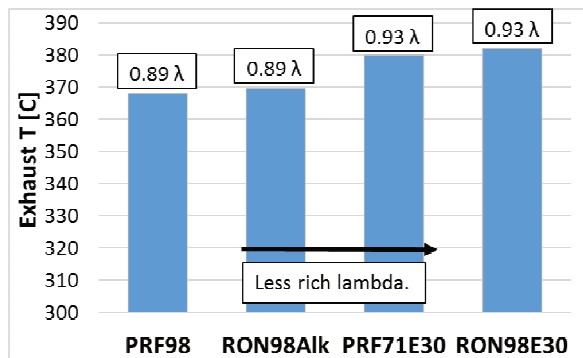
Fig. 6. Measured exhaust gas temperatures at RON conditions for each fuel
