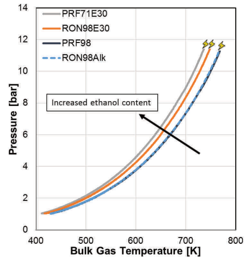
Fig. 7. Pressure-temperature trajectory from IVC to spark timing for each fuel at RON rating conditions
