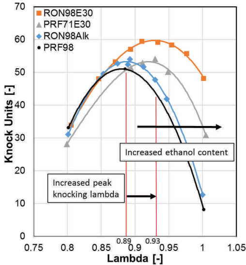
Fig. 1. ASTM knockmeter readings for lambda sweep from 0.8 to 1.0 for each fuel
