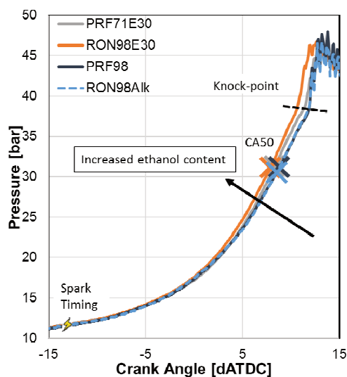
Fig. 8. Cylinder pressure from spark timing to combustion knock for each test fuel at RON rating conditions
