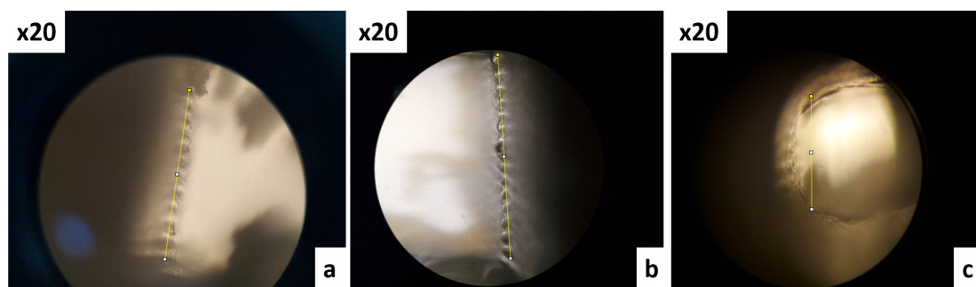
Fig. 1. Optical microscope ( \times 20 ) images of the central channel of the a) Original microsystem; b) Vapor- treated microsystem; c) In- situ surface treated microsystem
