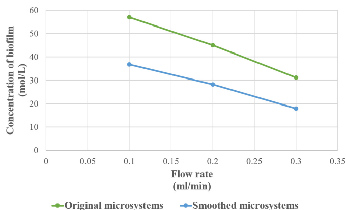
Fig. 8. Comparative chart of the biofilm concentration in original and in-situ surface treated microsystem versus of flow rate
