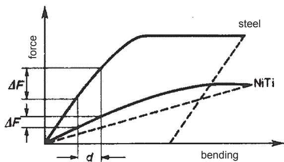
Fig. 15. Deformation forces for wires from NiTi and of austenitic stainless steel [1, 3]
