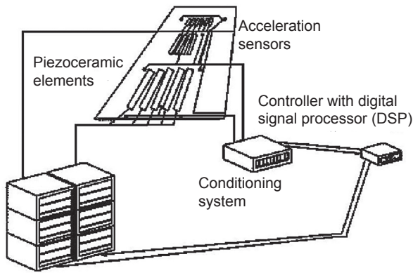
Fig. 4. Vibration Reduction Scheme of the tail of the aircraft
