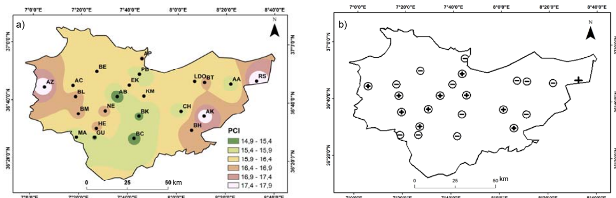
Fig. 5. Spatial distribution in the study region over the period 1970–2010 of the: a) monthly precipitation index ( PCI ), b) PCI trends (if the trend is non-significant, the plus or minus signs are circled); station codes as in Tab. 1; source: own study
