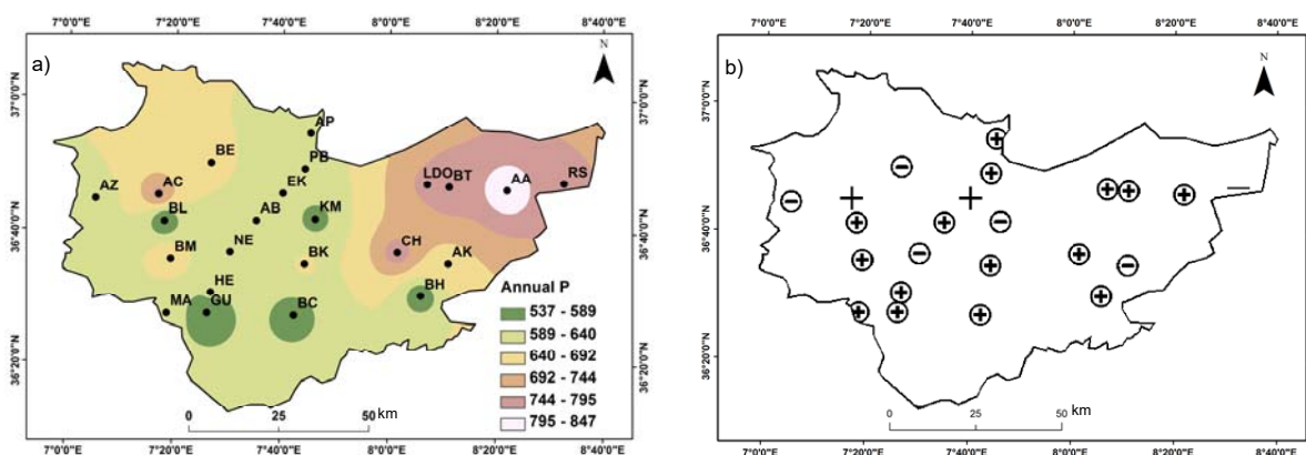
Fig. 3. Spatial distribution in the study region during 1970–2010 of: a) annual precipitations, b) trends for annual precipitation (if the trend is non-significant, the plus or minus signs are circled); station codes as in Tab. 1; source: own study
