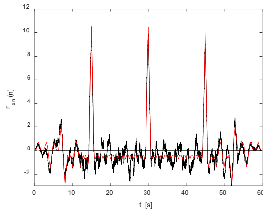
Figure 12. Functions of correlation of three analogue MLS's (red - without noise, black - with noise) (parameters as in Fig. 11, \sigma = 7 ).
