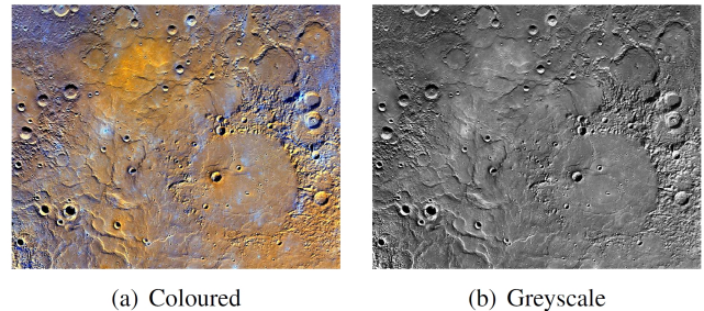
Fig. 4. Mercury Surface Map, NASA [4]. Colours were added to distinguish between rock types.
