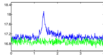
Fig. 14. Temperature time history plot obtained during vibrothermographic test. Blue curve represents the damaged area (1), green curve represents sound area (3)
